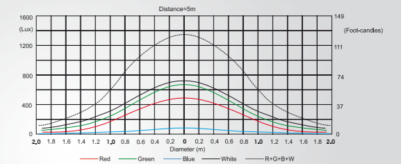
Illuminance distribution
